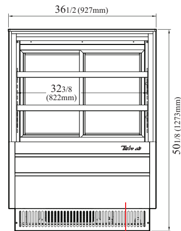
FRONT VIEW Power Cord (Back of the product)
