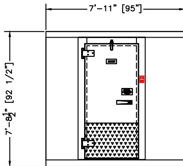
ELEVATION LEFT HINGE
