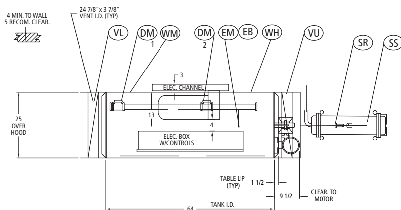
ELECTRIC TANK HEAT PTS. SIZE DESCRIPTION DM 2" NPT (F) DRAIN, MACHINE WASTE: LEAVE UNUSED PORTS PLUGGED WC 3/4" NPT (F) WATER SUPPLY: COLD AS AVAILABLE WM 3/4" NPT (F) WATER SUPPLY: 140° MIN. TANK FILL WH 3/4" NPT (F) WATER SUPPLY: 121 GALS./HR. @ 20 PSI WITHOUT BOOSTER 180°F. MIN WITH 15KW BOOSTER 140°F. MIN WITH 30KW BOOSTER 110°F. MIN EM ELECTRICAL REQ. 1. WASH PUMP MOTOR.....2 HP 2. RINSE PUMP MOTOR.....2 HP 3. CONVEYOR MOTOR.....1/4 HP 4. WASH TANK HEAT.....15 KW 5. RINSE TANK HEAT.....15 KW EB ELECTRICAL REQ. ONE (1) FEEDER SIZED FOR: 30KW BOOSTER VL NOTED VENT, LOAD END: RECOM. MIN. DRAW = 200 CFM VU NOTED VENT, UNLOAD END: RECOM. MIN. DRAW = 400 CFM
