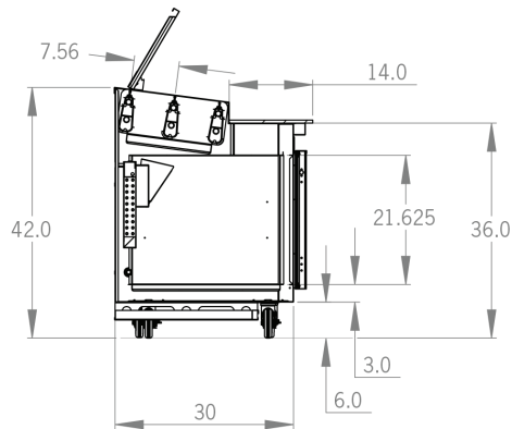
Section View
