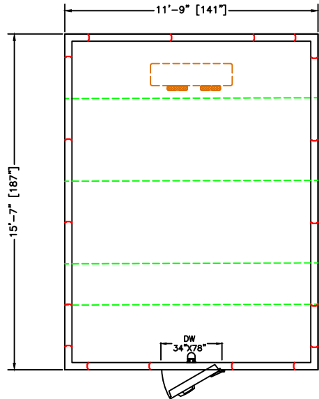
PLAN VIEW RIGHT HINGE SELECT
