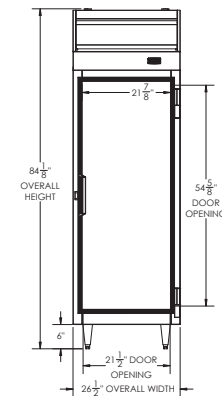
ELEVATION VIEW
