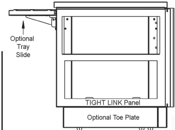
End View ▲
