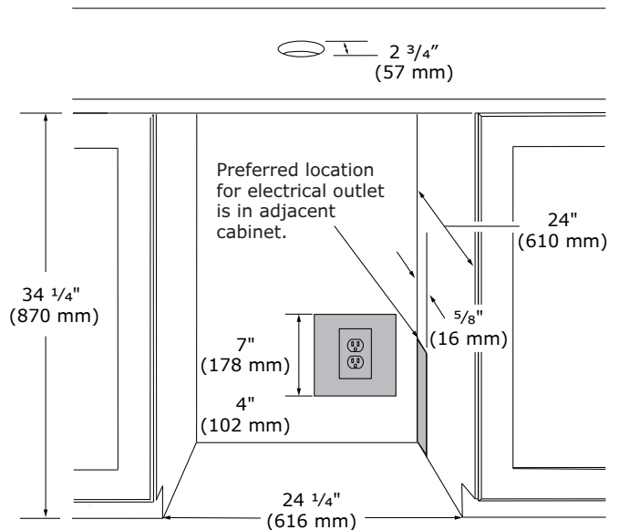
Cabinet Cut-Out
