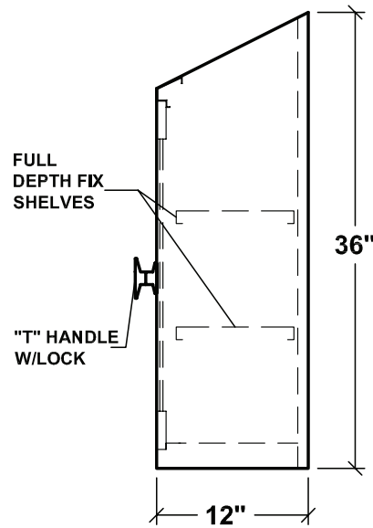
SIDE ELEVATION
