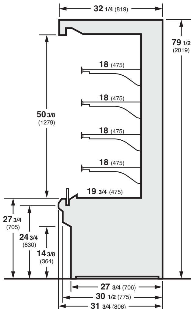
Cross Section
