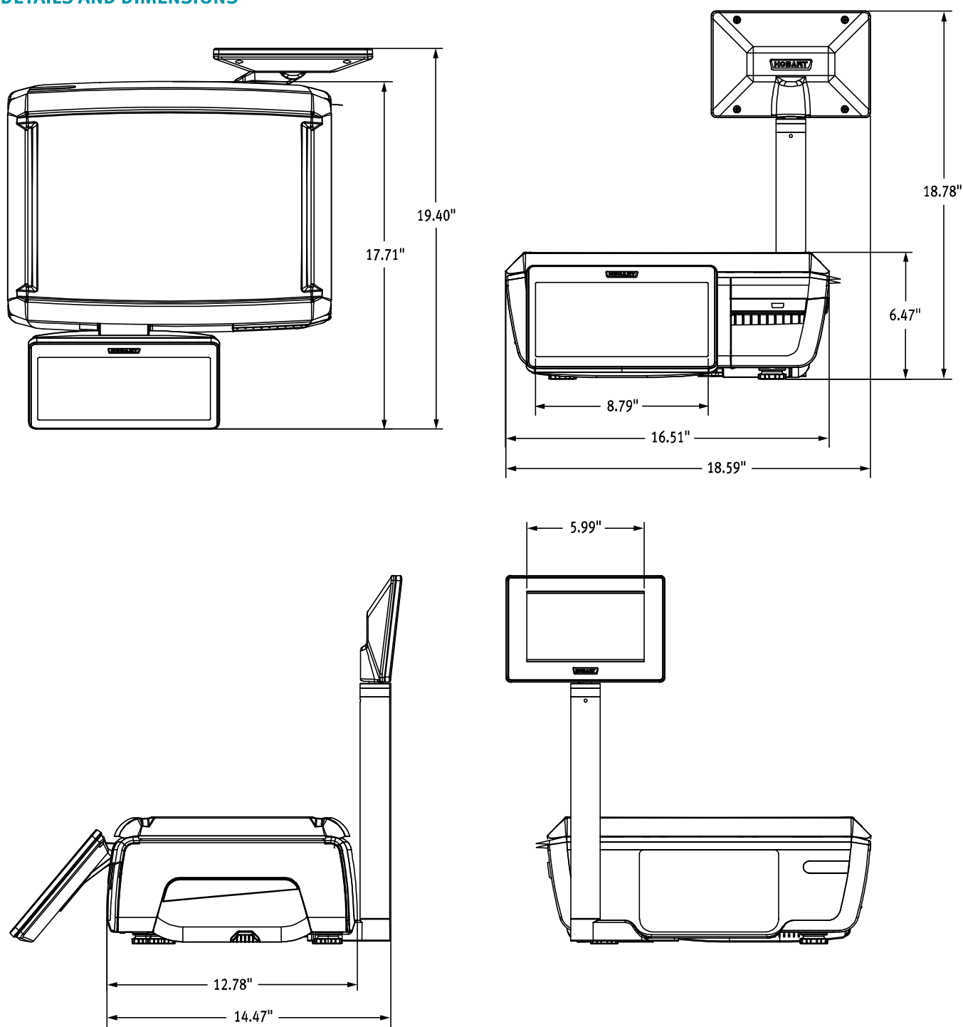
GTs 10.1" Operator Display, 7" Elevated Customer Display
