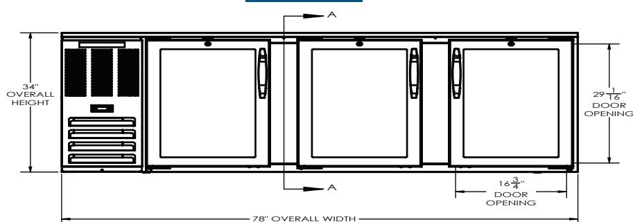
ELEVATION VIEW
