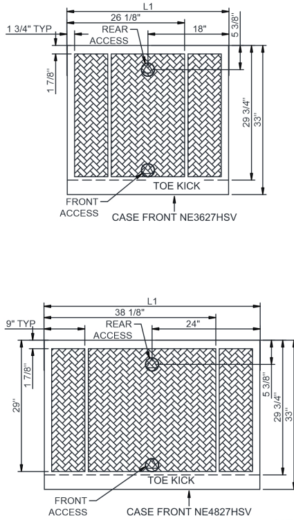
PLAN VIEW
