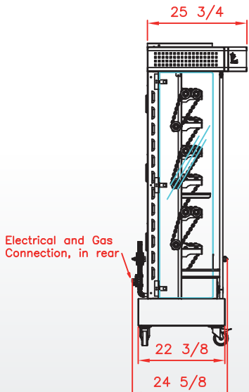
Side view Rotisserie with roof
