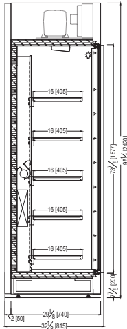
OPTIONAL: TOP MOUNTED CONDENSING UNIT
