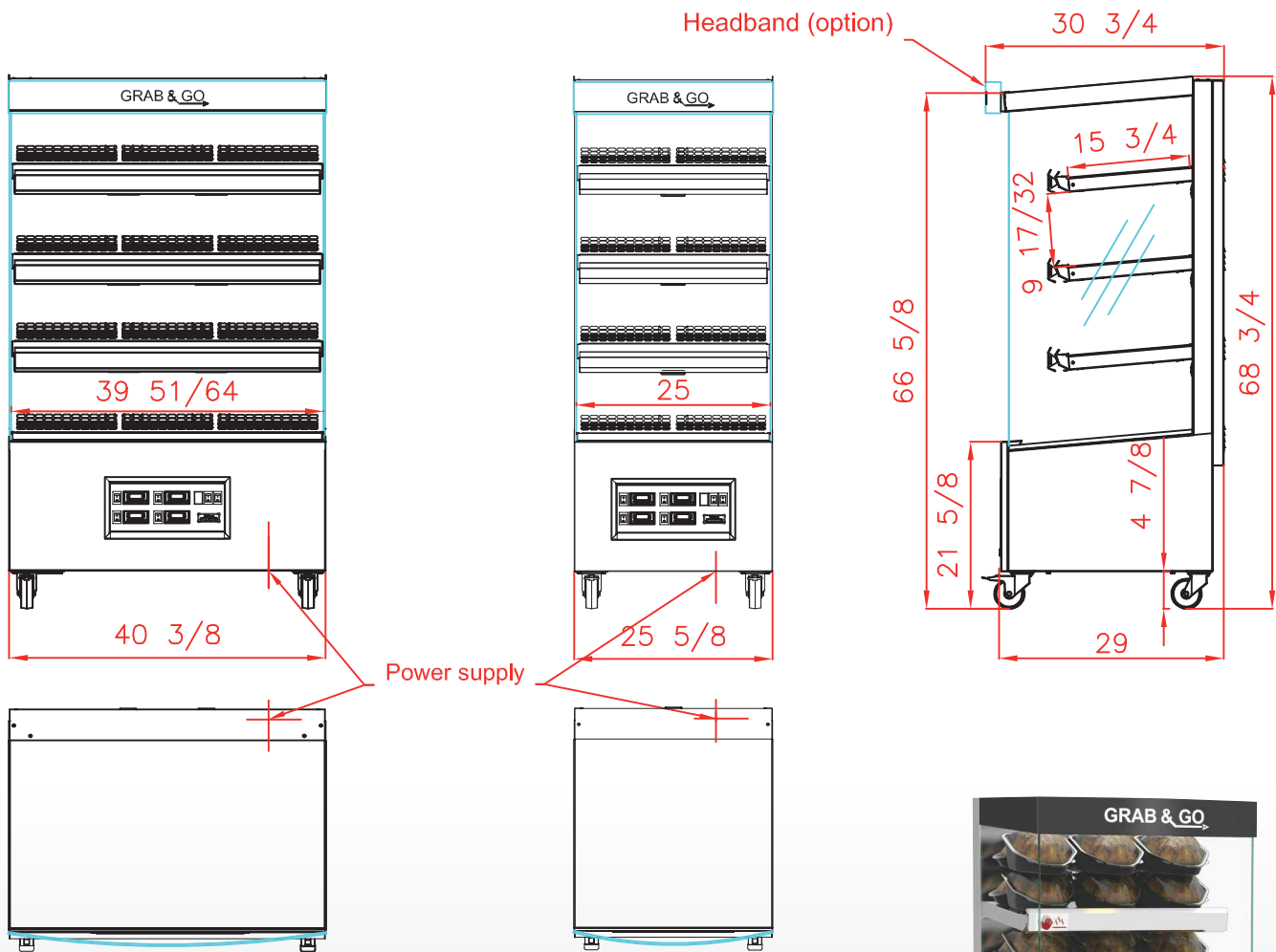
Front view 10MCV4LS.I
