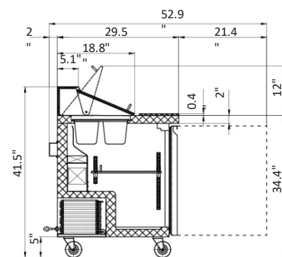
Side Section
