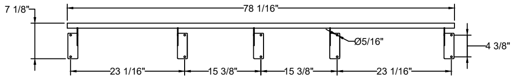
FRONT ELEVATION
