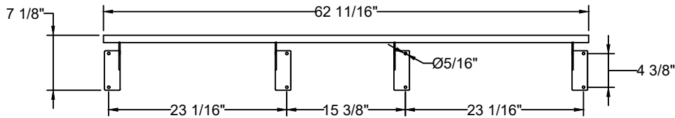
FRONT ELEVATION
