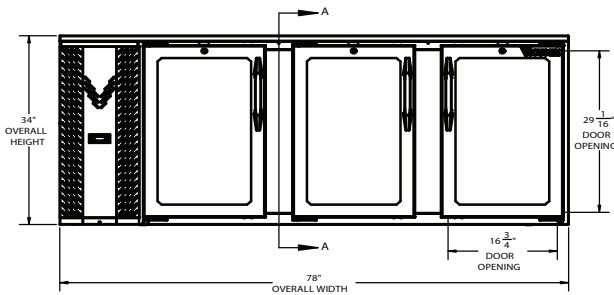
ELEVATION VIEW
