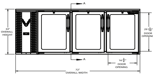
ELEVATION VIEW
