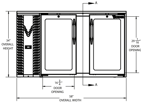
ELEVATION VIEW
