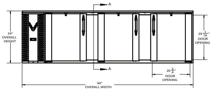
ELEVATION VIEW
