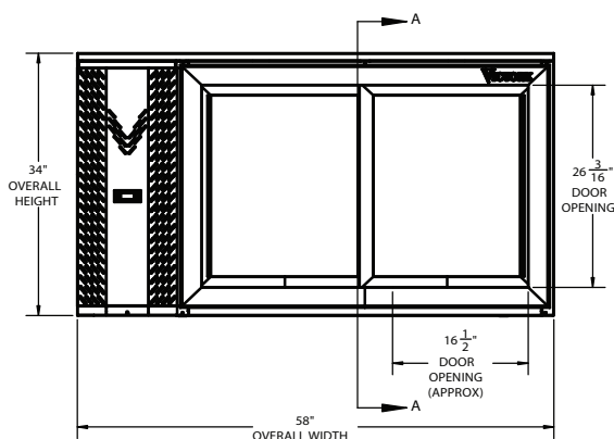
ELEVATION VIEW
