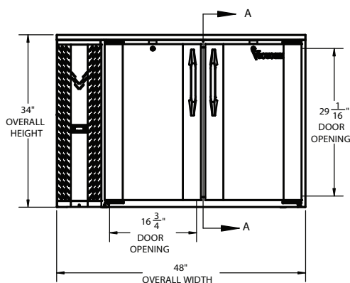
ELEVATION VIEW
