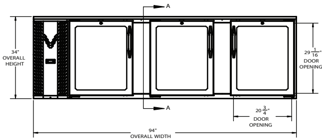
ELEVATION VIEW
