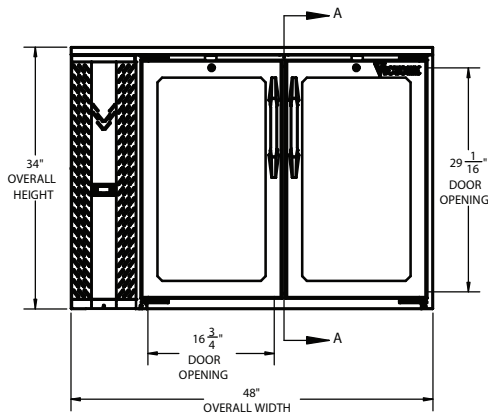
ELEVATION VIEW
