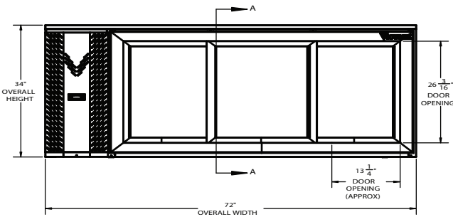
ELEVATION VIEW
