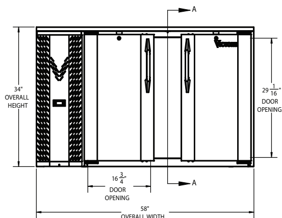
ELEVATION VIEW
