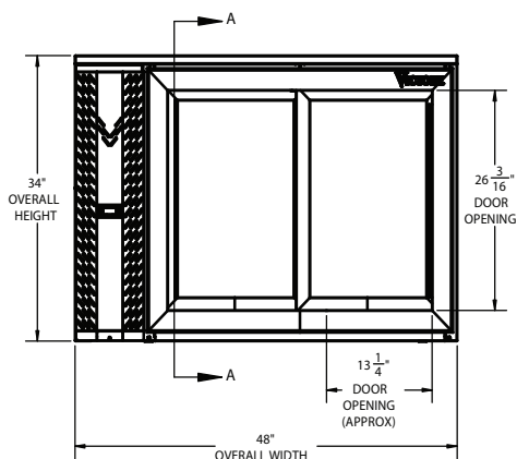
ELEVATION VIEW
