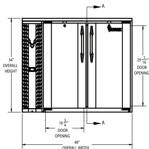
ELEVATION VIEW
