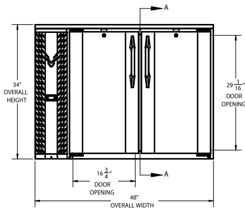
ELEVATION VIEW
