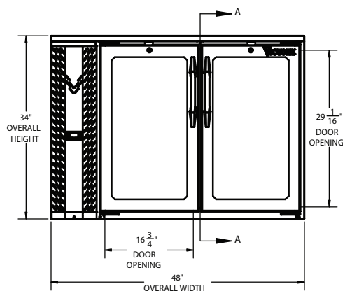
ELEVATION VIEW
