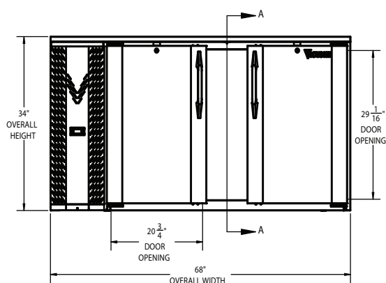
ELEVATION VIEW
