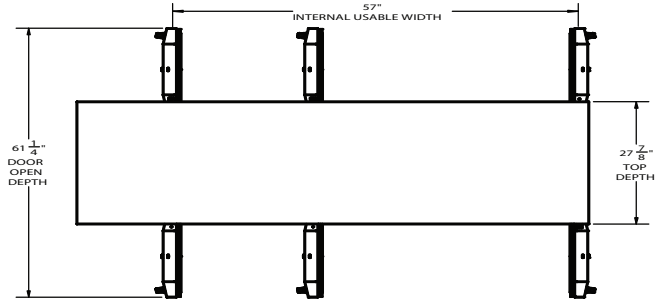
PLAN VIEW
