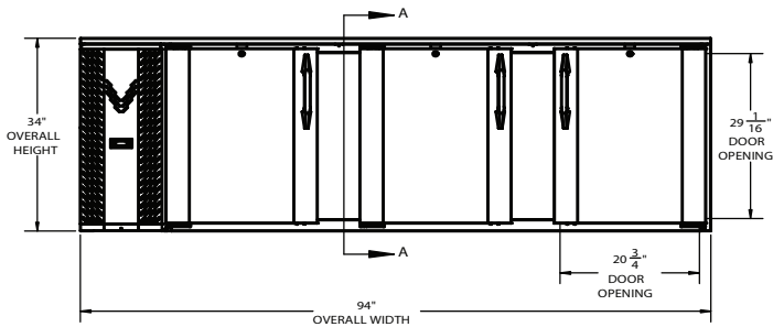
ELEVATION VIEW
