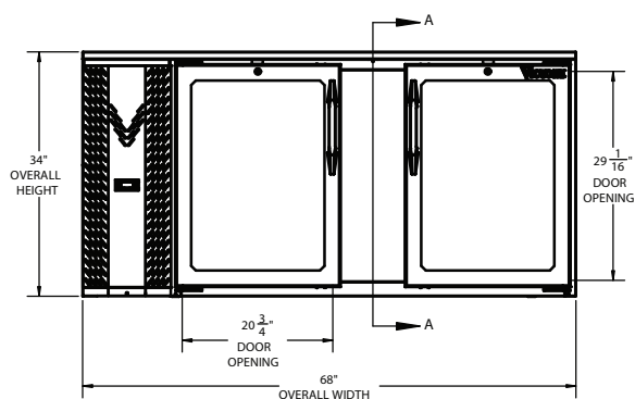
ELEVATION VIEW
