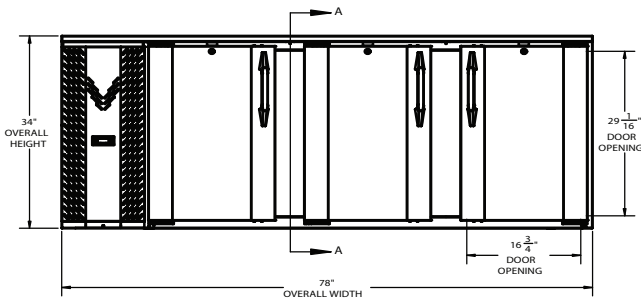
ELEVATION VIEW
