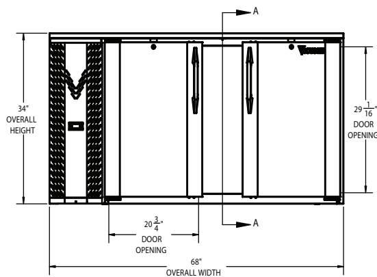
ELEVATION VIEW
