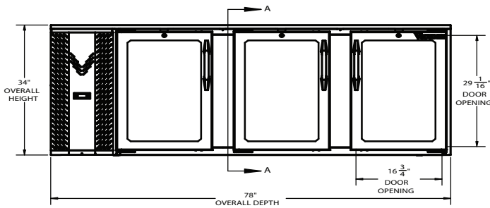
ELEVATION VIEW
