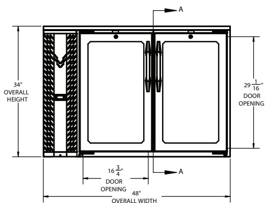
ELEVATION VIEW
