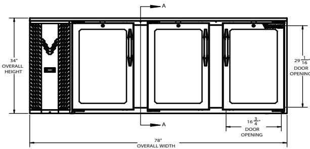
ELEVATION VIEW
