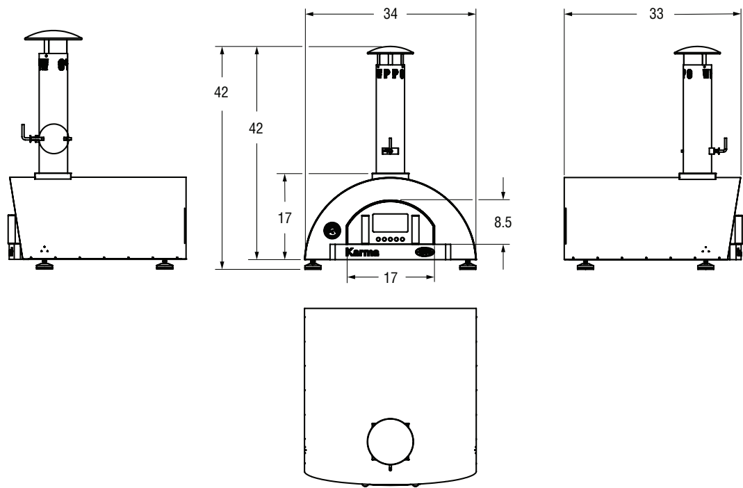
Figure X. Dimensions: 32in. Oven with Cart
