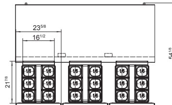
Rear grate
