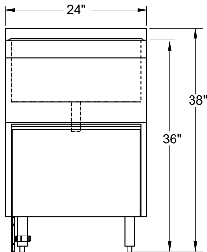
FRONT ELEVATION
