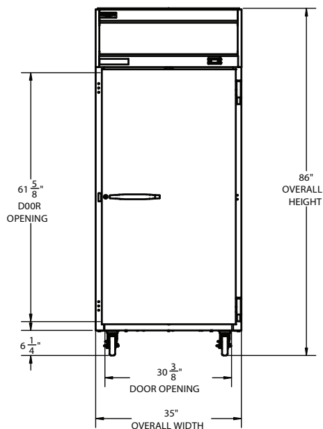
ELEVATION VIEW
