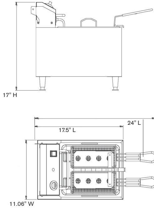
PF16E-C
