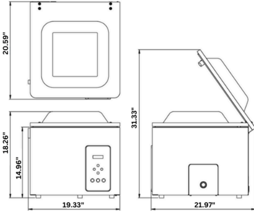
Unit Dimensions
