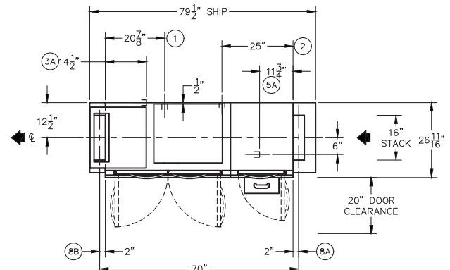
Plan View: Right to Left Model
