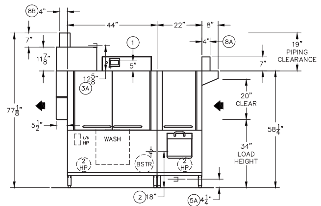
Front View: Right to Left Model
