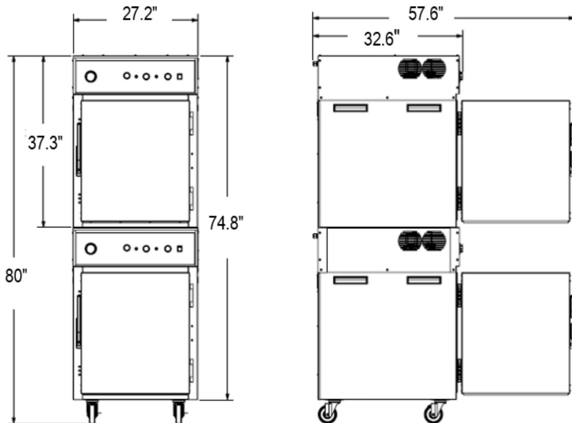
CC-CHC-2 Dimensions
