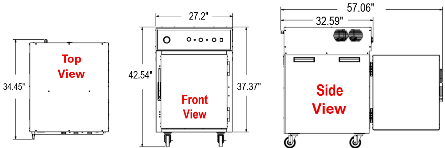
CC-CHC-1 Dimensions
